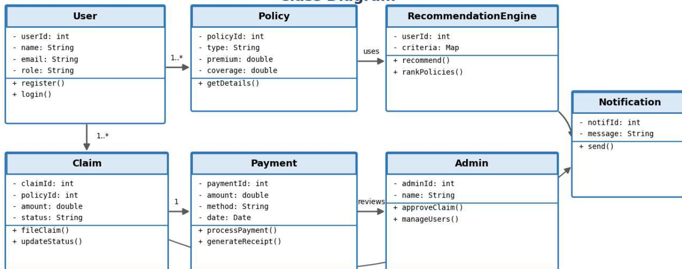
Class Diagram
